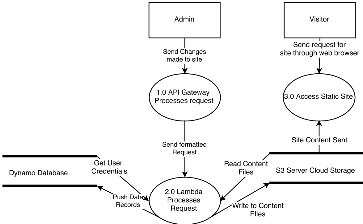
CMS DFD Level 0
